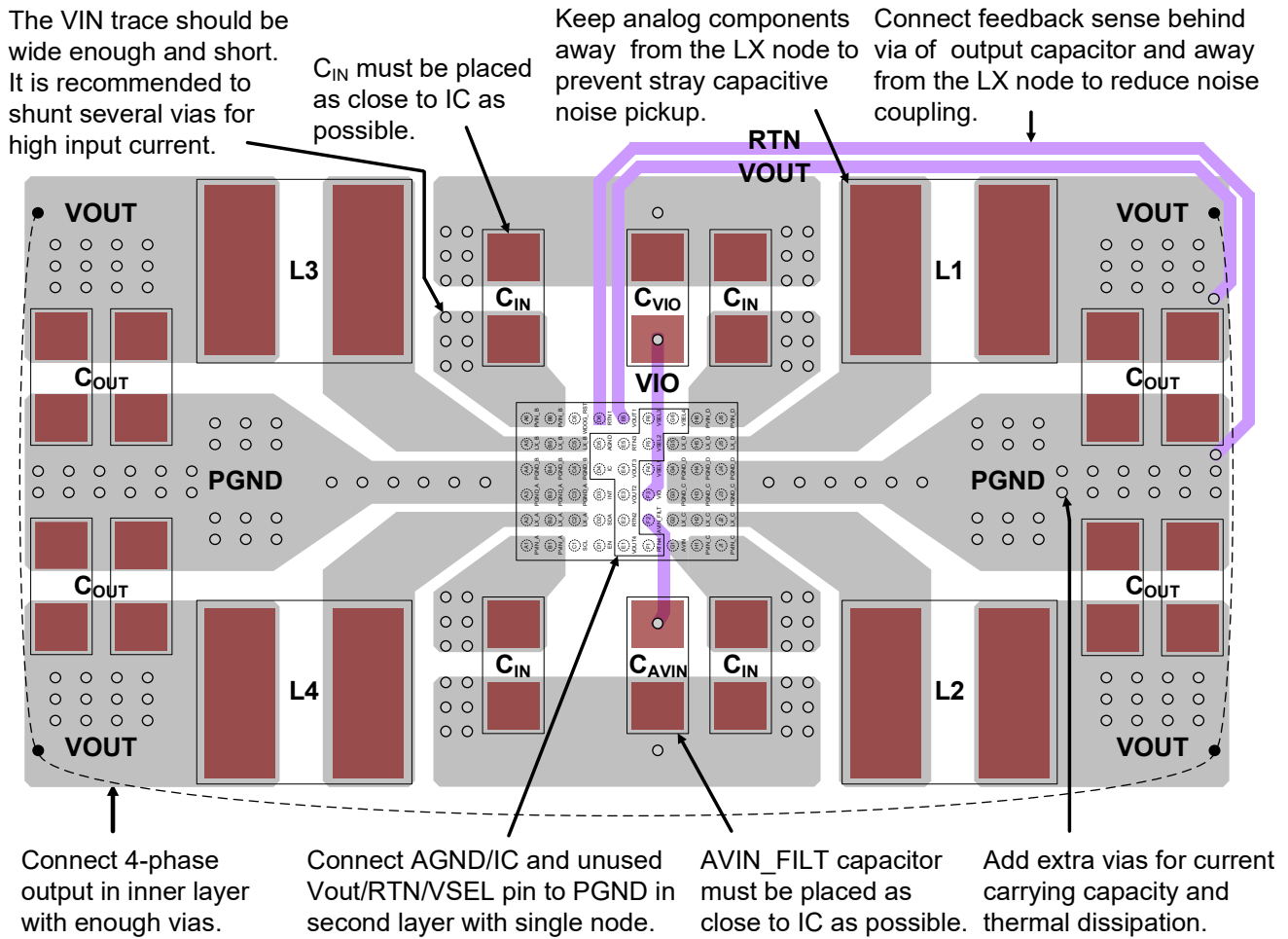
Figure 11. RTQ5756D Layout Guideline
