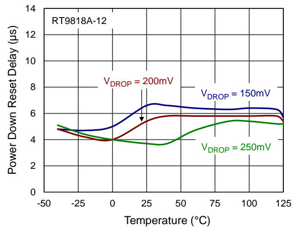
Power-Down Reset Delay vs. Temperature
