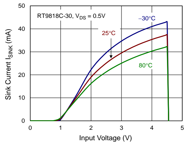
N-CH Driver Sink Current vs. Input Voltage
