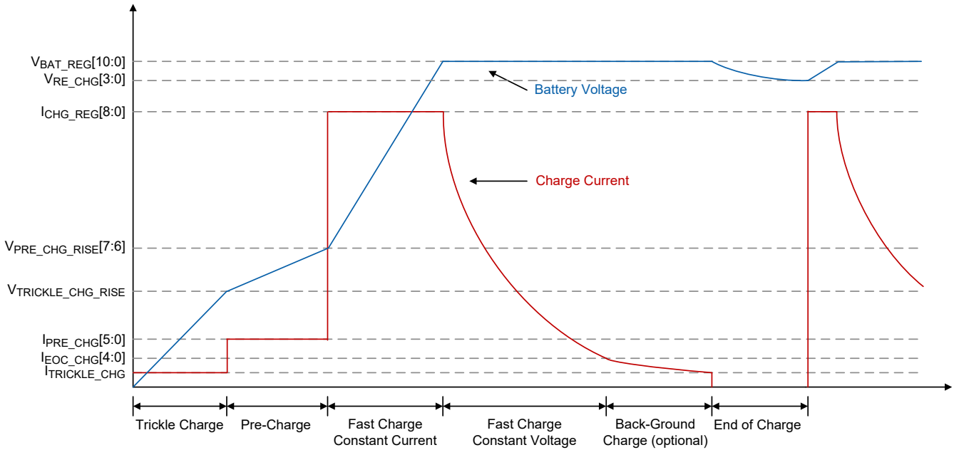
Figure 1. Charging Profile
