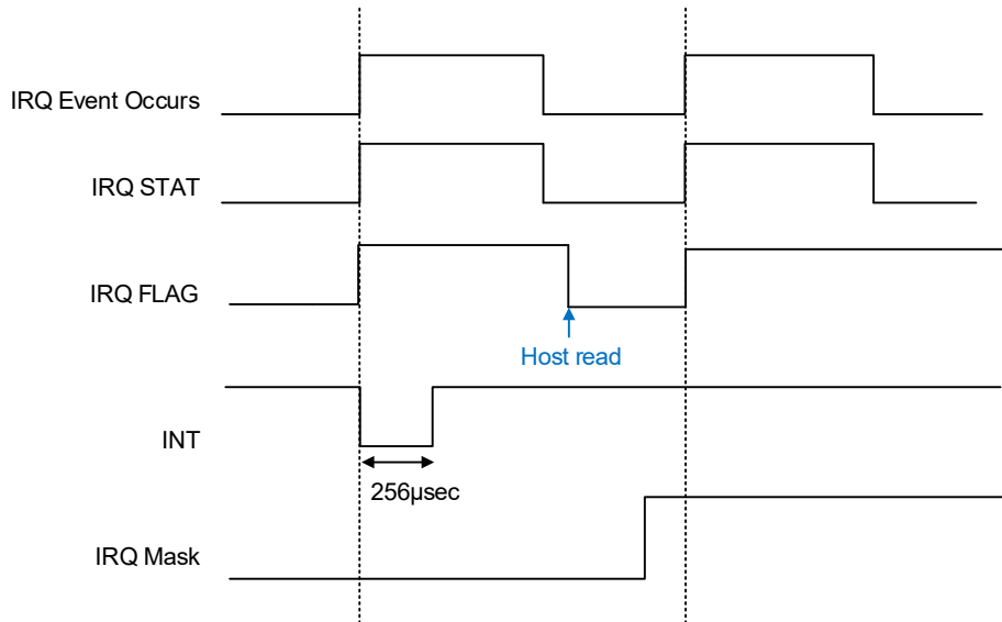
Figure 8. The Operation of Flag, Status, INT, and Mask
