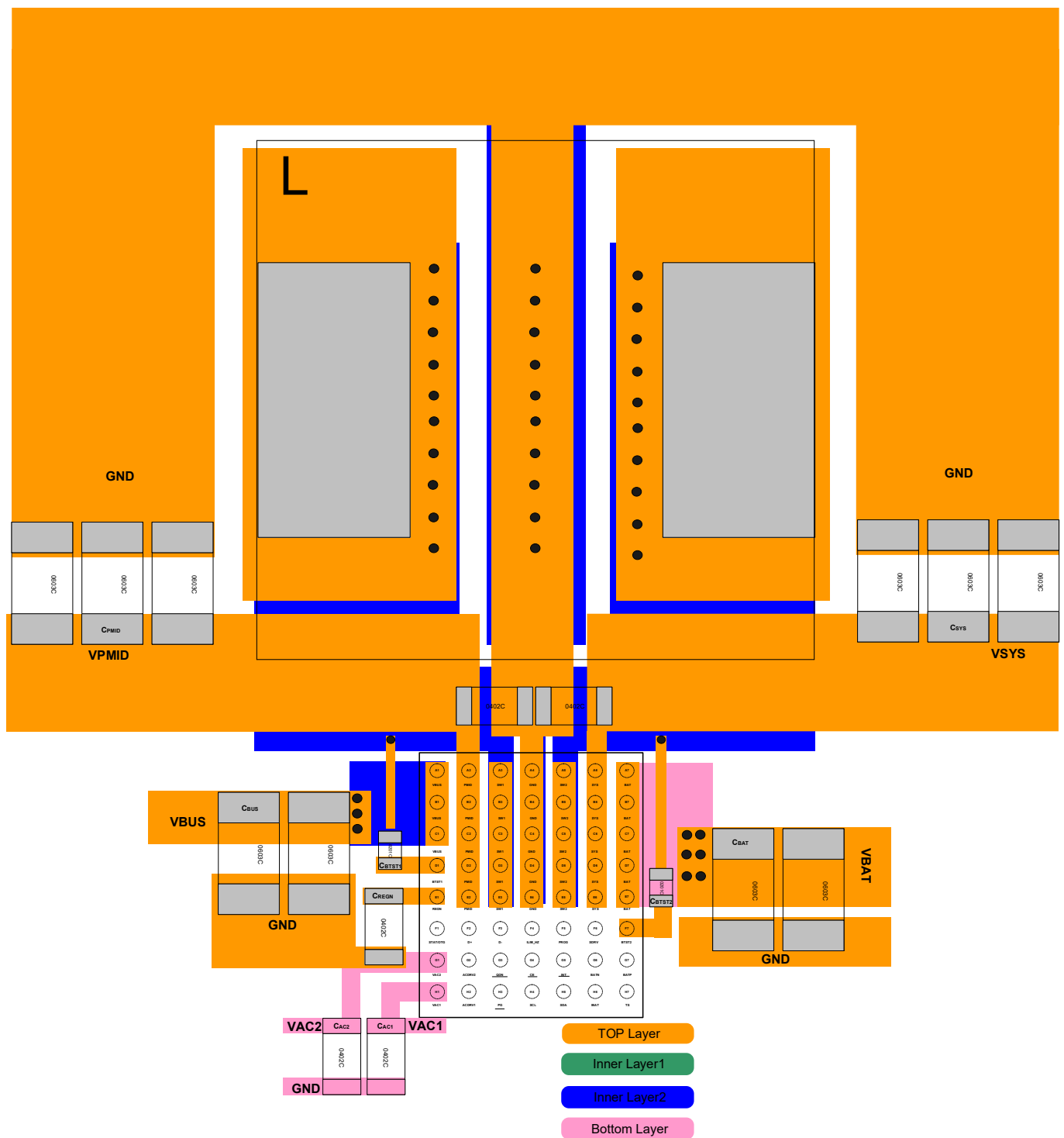
Figure 12. PCB Layout Guide
