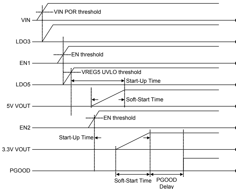
Figure 4. RT8249D Timing
