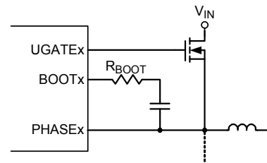
Figure 3. Increasing the UGATEx Rise Time
