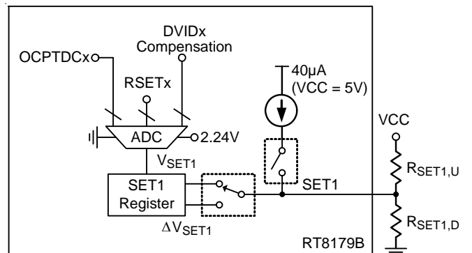
Figure 6. SET1 Pin Setting
