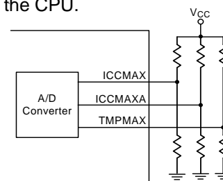
Figure 3. ADC Pins Setting
