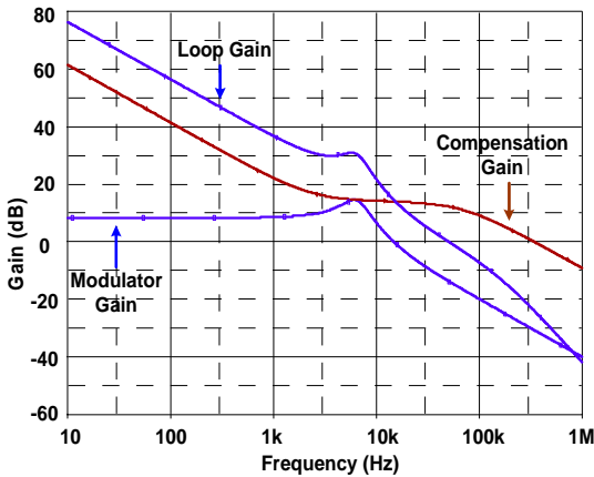
Figure 6. System Gain Bode Plot
