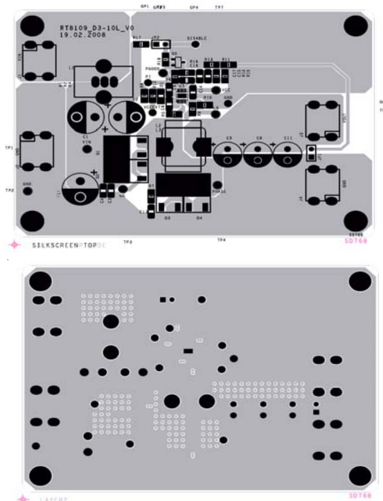
Figure 7. PCB Layout
