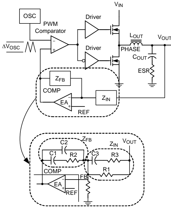
Figure 4. Control Loop for Voltage Mode Buck Converter
