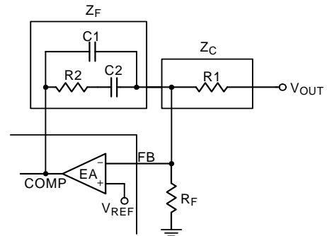
Figure 5. Type II Compensator
