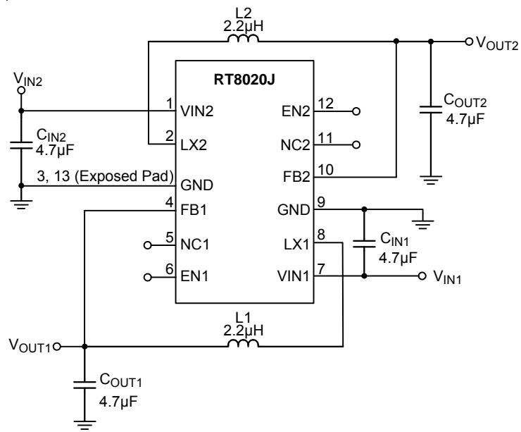
Figure 2. Fixed Voltage Regulator
