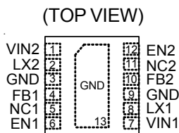
WDFN-12L 3x3
