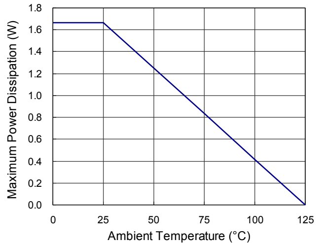
Figure 4. De-rating Curves for RT8020J Package
