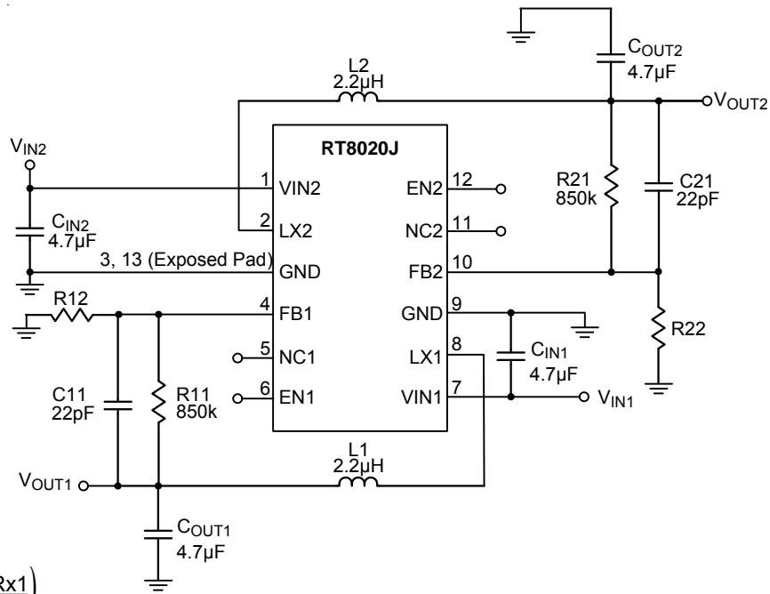
Figure 1. Adjustable Voltage Regulator
