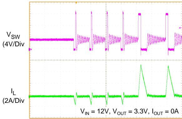
Time (2μs/Div)
