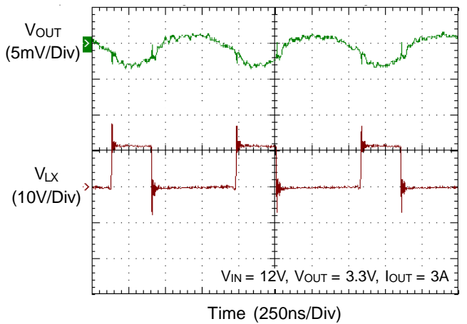
Ripple Voltage
