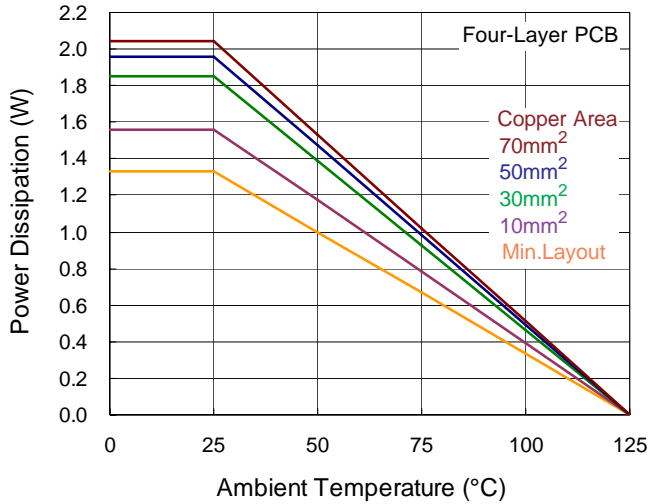
Figure 8. Derating Curves for RT7256A Package
