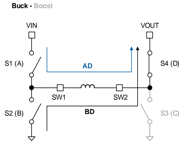
Figure 1. Buck Operation
