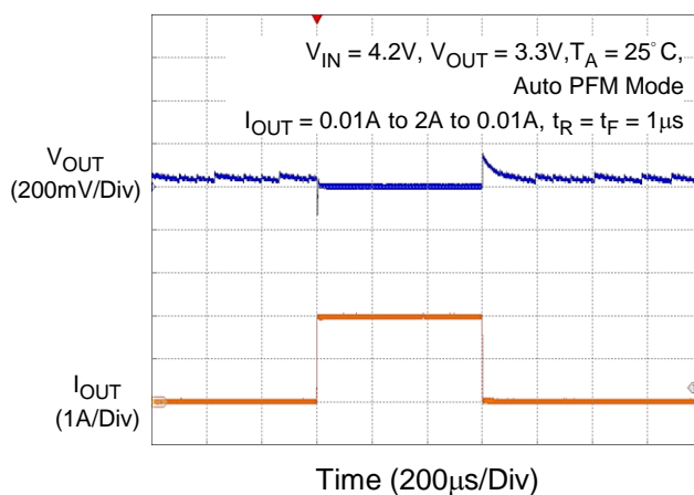
Load Transient Response (Buck)
