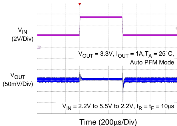
Line Transient Response (Heavy Load)
