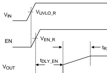
Figure 4. Soft-Start Sequence
