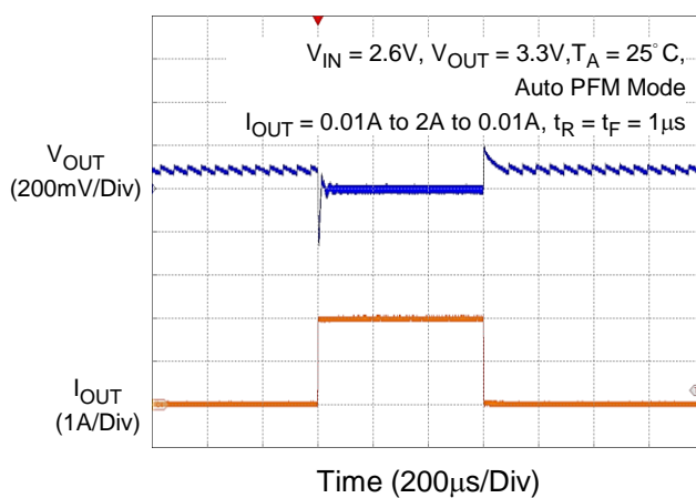
Load Transient Response (Boost)
