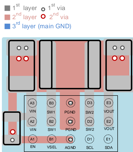
Figure 8. Layout Guide
