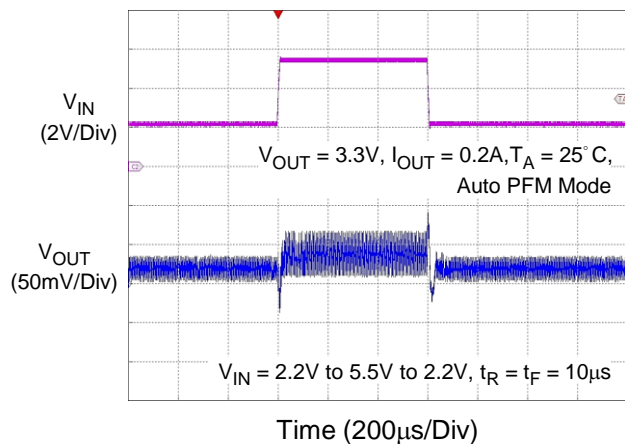
Line Transient Response (Light Load)
