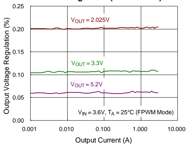
Load Regulation (FPWM Mode)
