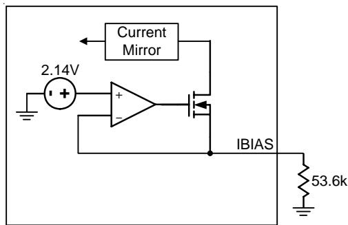
Figure 5. IBIAS Setting
