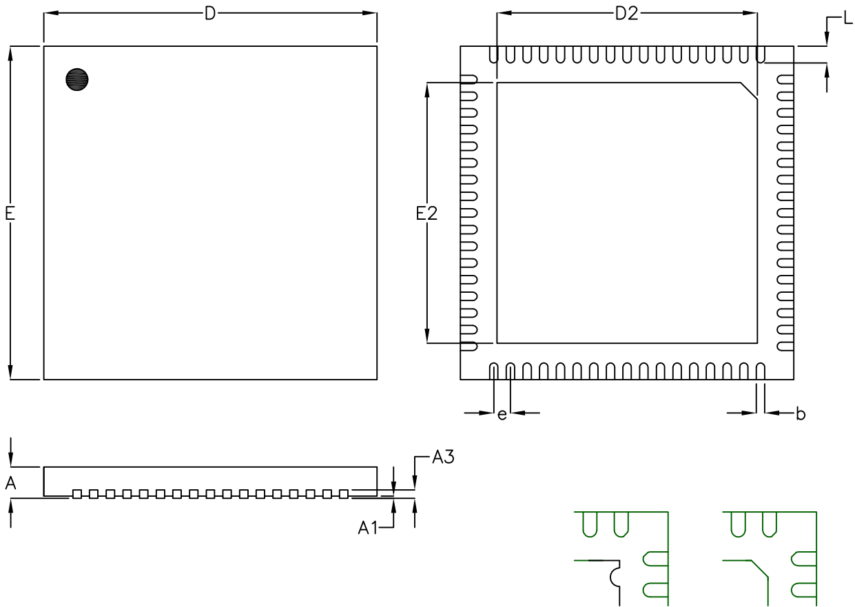
Pin #1 ID and Tie Bar Mark Options
