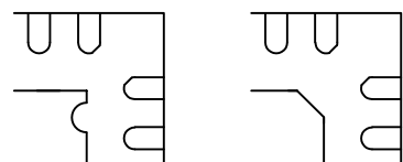
Pin #1 ID and Tie Bar Mark Options
