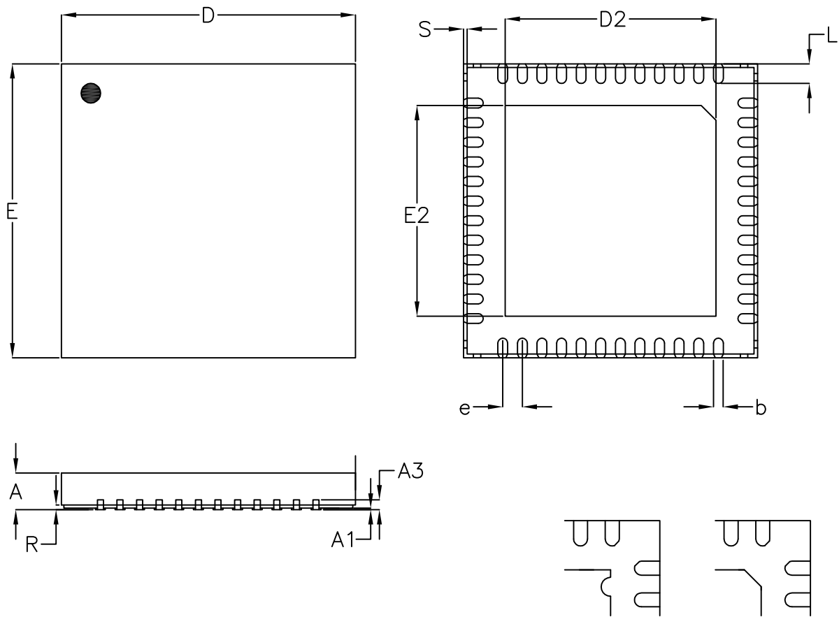
Pin #1 ID and Tie Bar Mark Options
